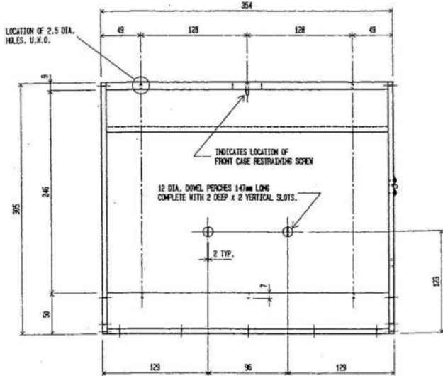
FRONT ELEVATION WIRE CAGING NOT SHOWN FOR CLARITY. REFER ELEVATION FOR WIRE CAGING DETAILS.
