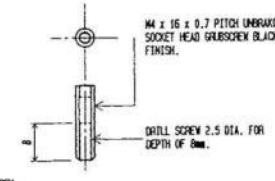
FRONT RESTRAINING SCREW SCALE 2:1
