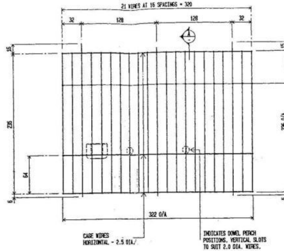
ELEVATION - WIRE CAGING NOTE: CASE WIRES - 2.0 DIA. / 2.5 DIA. TO BE CHROMIUM PLATED IN ACCORDANCE WITH SHOWCASE SPECIFICATION.
