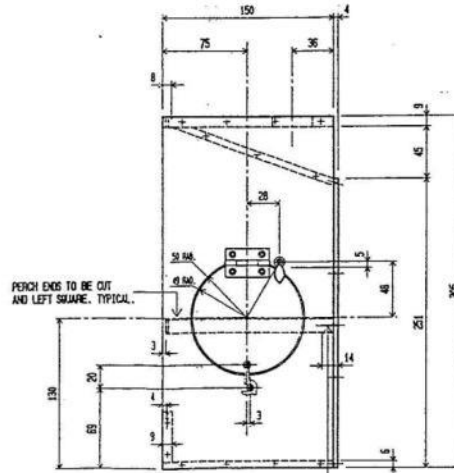
ELEVATION - WIRE CAGING
