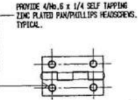
40 x 25 CABINET SERIES BUTT HINGES SCALE 1:1
